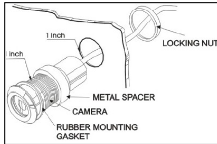
Typical Bulkhead Mount
